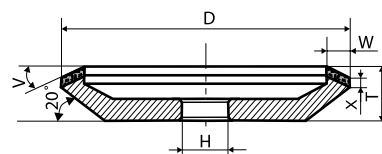
12V5-20 D*T*W*X*V*H
